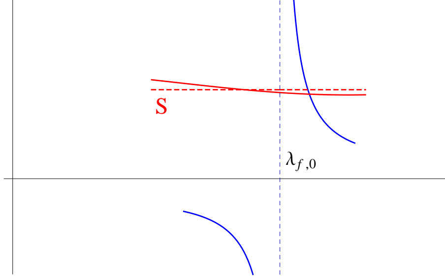
Figure 9: The statement of Lemma 5.14 graphically explained. The lefthand side of (5.19), which is singular at \lambda = \lambda_{f,0} , is indicated in blue, the righthand side of (5.19) is indicated in red and its approximation S (5.18) by the dashed line.
