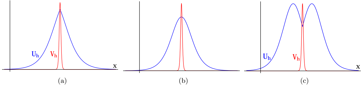
Figure 3: The stationary homoclinic pulse \Gamma_h(x) = (U_h(x), V_h(x)) as a solution to (1.2) for x_* > 0 (3a), x_* = 0 (3b) and x_* < 0 (3c), as studied in the companion paper [36].
