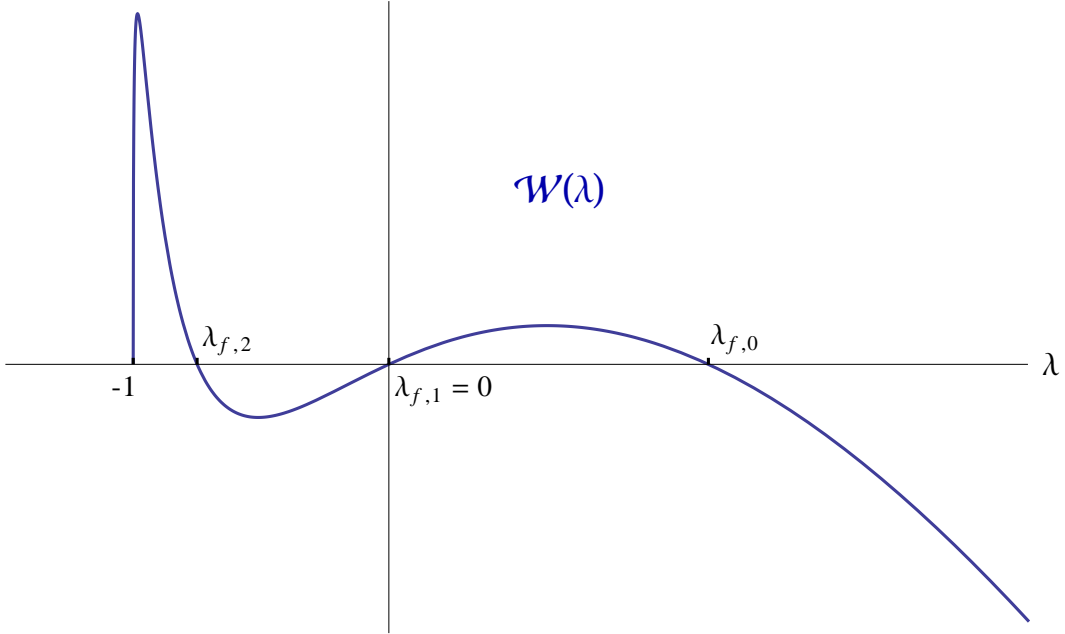
Figure 4: A sketch of the Wronskian \mathcal{W}(\lambda) associated to (3.12) in the case of the model problem (1.2), for \lambda \in \mathbb{R} .
