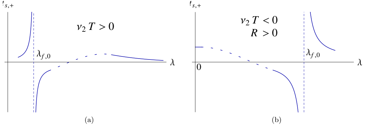
Figure 8: An illustration of the proof of Lemma 5.11 (8a) and Lemma 5.12 (8b). The (singular) behaviour of t_{s,+} near \lambda = \lambda_{f,0} is determined by the sign of \nu_2 T (Lemma 5.1). In (a), this leads to at least one root of t_{s,+} to the right of \lambda_{f,0} > 0 since t_{s,+} \sim e^{-2y_*\lambda} as \lambda \rightarrow \infty . In (b), t_{s,+} has to cross the horizontal axis in the interval \lambda \in (0, \lambda_{f,0}) at least once if R > 0 .
