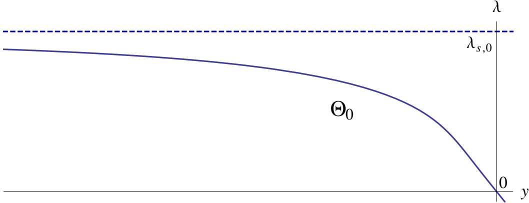
Figure 6: The zero set \Theta_0 = \{(\lambda, y_0) \mid \lim_{\varepsilon \rightarrow 0} \theta_{s,-}(y_0, \lambda, \varepsilon) = \frac{\pi}{2}\} .
