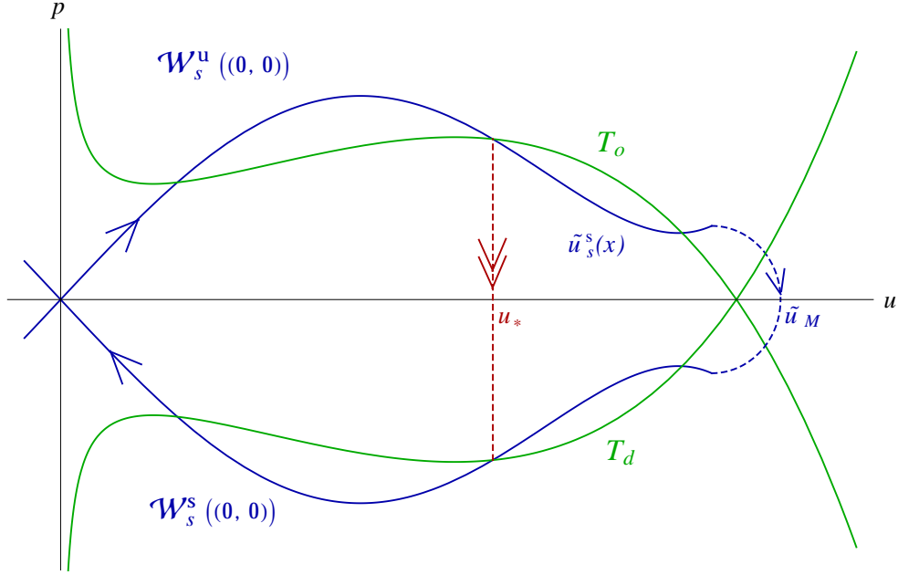
Figure 2: The slow manifold with its dynamics as in Figure 1, but altered for u > u_* in such a way that the (new) slow stable and unstable manifolds \tilde{W}_s^s((0,0)) and \tilde{W}_u^s((0,0)) intersect at (\tilde{u}_M, 0) .
