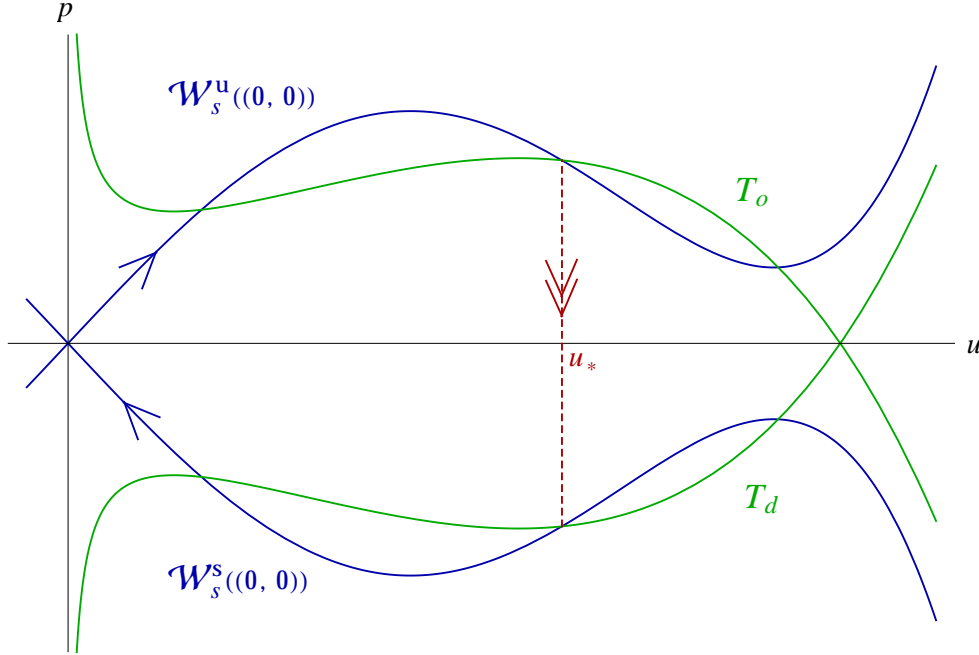
Figure 1: The dynamics on the slow manifold \mathcal{M} , governed by (2.13). The jump through the fast field is indicated by a red dashed line.
