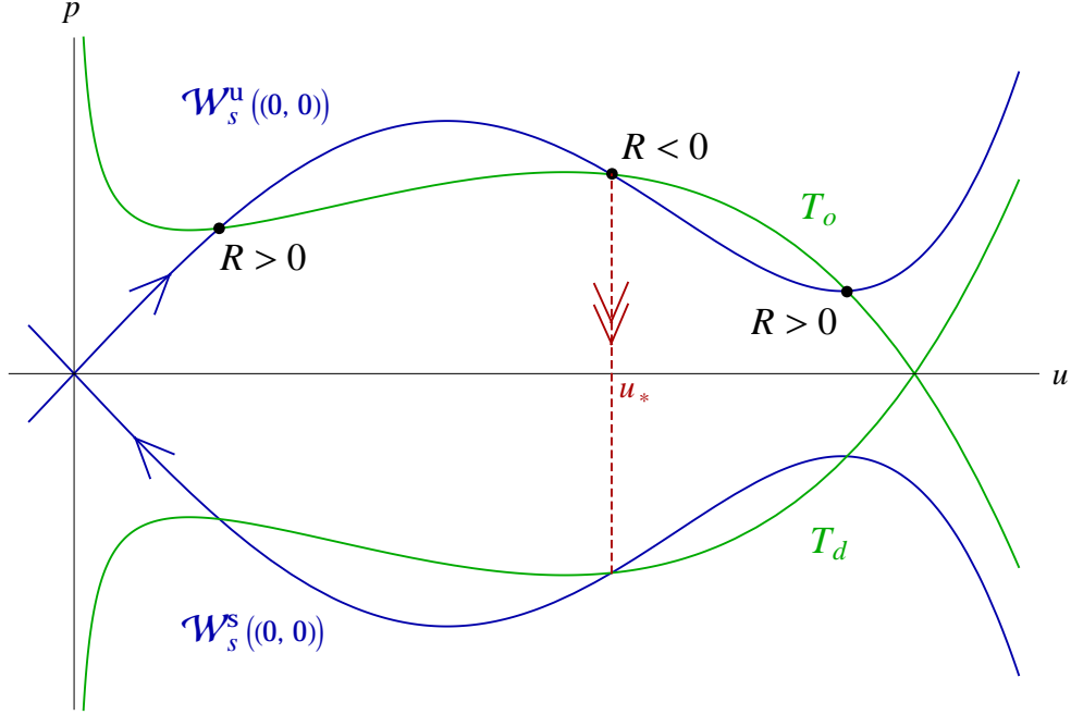
Figure 7: The coefficient R (5.17) interpreted geometrically as the relative slope of T_o with respect to \mathcal{W}_s^u((0, 0)) at their intersection point. Only the homoclinic pulse associated to the second intersection can be stable (Lemma 5.12).
