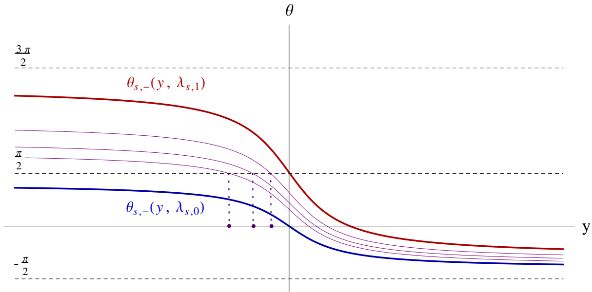
Figure 5: The ordering of \theta_{s,-}(y; \lambda) , depicted for \lambda_1 \leq \lambda \leq \lambda_0 . The intersections with the line \theta = \frac{\pi}{2} are also indicated; for these values of \lambda , each of these intersections is to the left of y = 0 .
